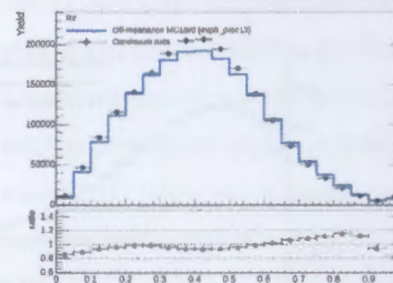
Figure 10: R_2 distribution before tuning.
