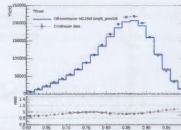
Figure 8: Thrust distribution before tuning.
