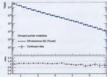
Figure 5: Charged particle multiplicity after tuning.
