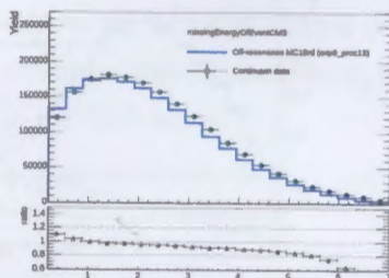
Figure 14: MissingEnergyOfEventCMS distribution before tuning.
