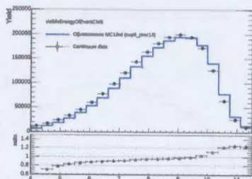
Figure 16: VisibleEnergyOfEventCMS distribution before tuning.
