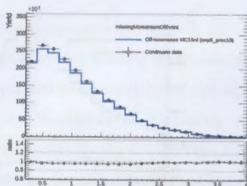
Figure 12: MissingMomentumOfEvent distribution before tuning.
