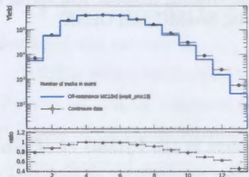
Figure 6: Number of tracks per event before tuning.
