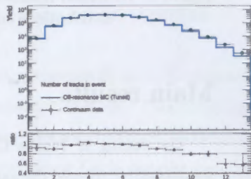
Figure 7: Number of tracks per event after tuning.
