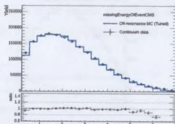
Figure 15: MissingEnergyOfEventCMS distribution after tuning.
