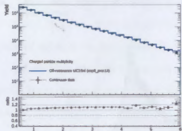
Figure 4: Charged particle multiplicity before tuning.
