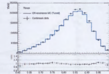
Figure 9: Thrust distribution after tuning.
