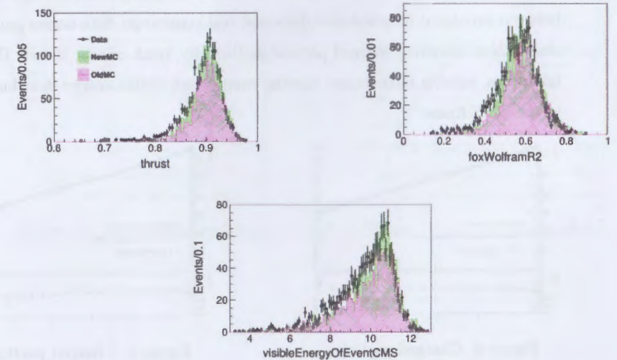
Figure 3: Validation results of thrust, Fox-Wolfram moment, and visible energy distributions comparing data, NewMC, and OldMC.
