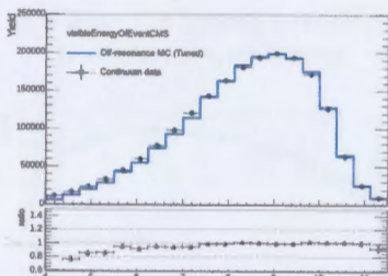
Figure 17: VisibleEnergyOfEventCMS distribution after tuning.
