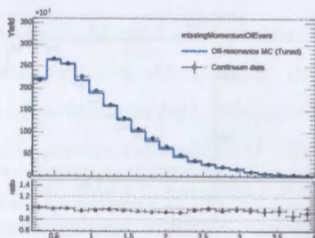
Figure 13: MissingMomentumOfEvent distribution after tuning.
