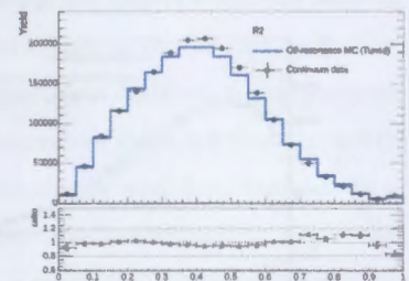
Figure 11: R_2 distribution after tuning.
